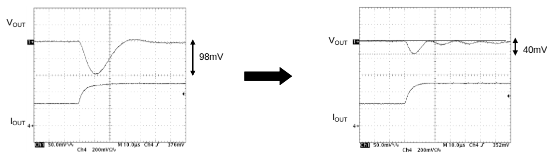
Figure 4. Comparison of transient response
