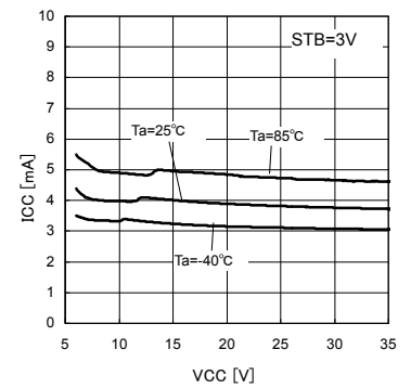
Fig.21 Circuit current-Supply voltage I_{out} = \text{No Load}
