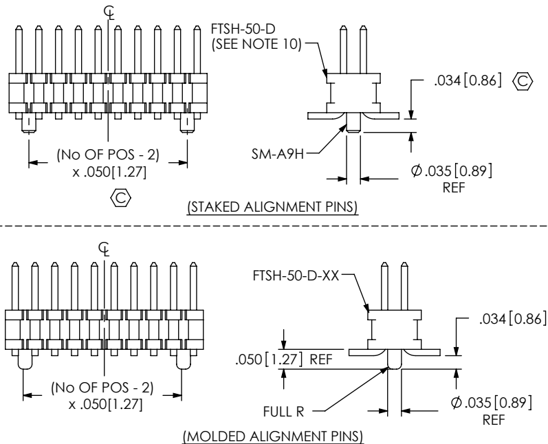
FIG 3 -A OPTION (DIFFERENT AS SHOWN, OTHERWISE SAME AS FIG 1) (6 POSITION MINIMUM FOR STAKED ALIGNMENT PINS) (3 POSITION MINIMUM FOR MOLDED ALIGNMENT PINS)
