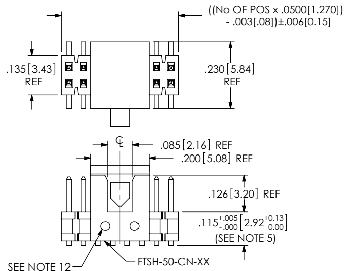
FIG 2 -K OPTION (LEAD STYLE -01 ONLY) S SHOWN, OTHERWISE S N 13, 17, 20 & 25 AVAILA -EJ OPTION)
