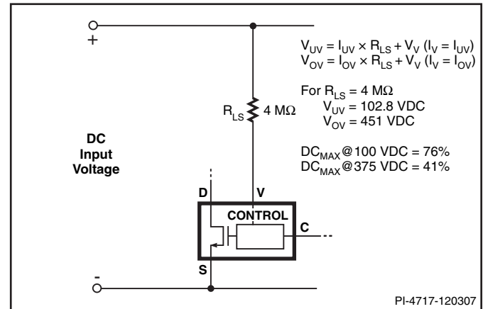
Figure 13. Line-Sensing for Undervoltage, Overvoltage and Line Feed-Forward.
