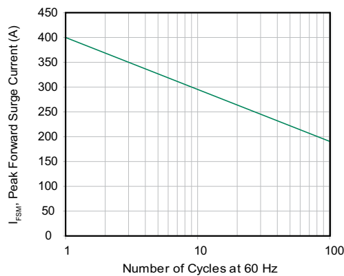
Figure 7 - Maximum Non-Repetitive Forward Surge Current
