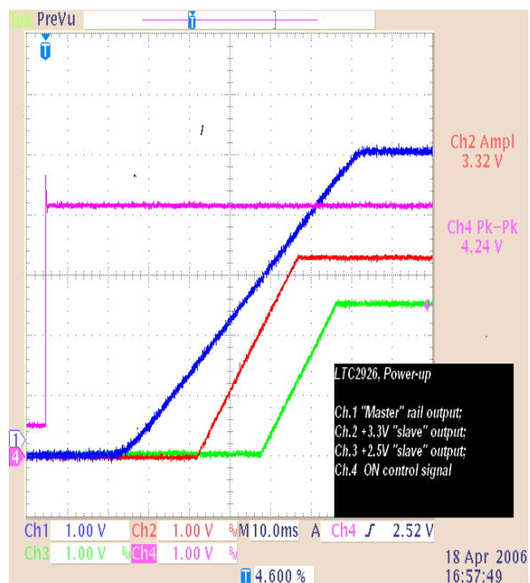
Figure 3. Power-up mode
