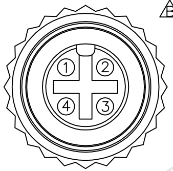
Conn.2 Pin Assignments Front View
