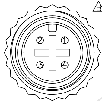
Conn.1 Pin Assignments Front View
