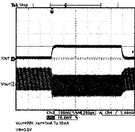
Load Transient
