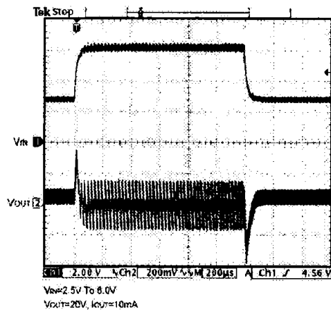
Line Transient
