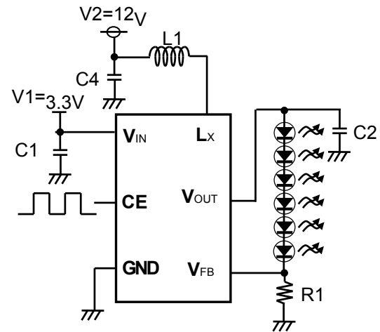
Fig 2. R1207N8xxB/C
