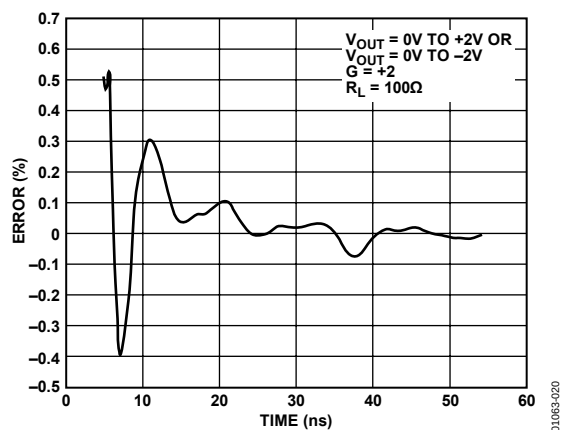
Figure 18. Settling Time
