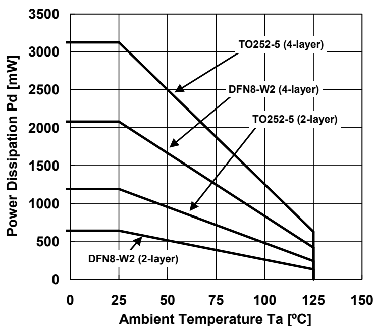
Figure 1 : Power Dissipation Derating Curve
