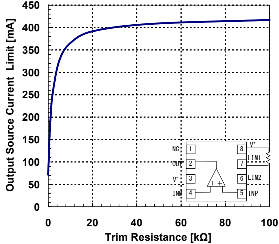
Output Source Current Limit vs. Current Limit Trim Resistance
