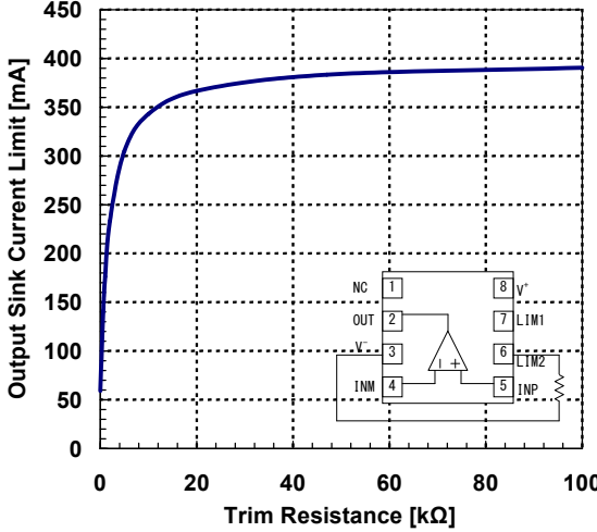
Output Sink Current Limit vs. Current Limit Trim Resistance
