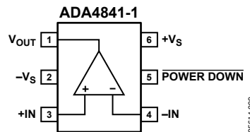
Figure 2. 6-Lead SOT-23 (RJ)
