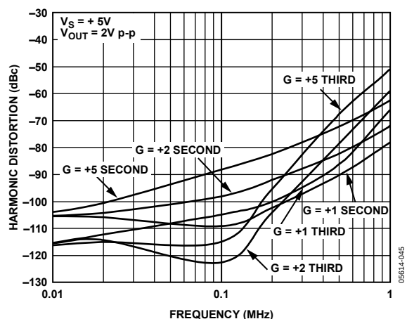
Figure 13. Harmonic Distortion vs. Frequency for Various Gains
