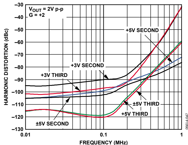
Figure 15. Harmonic Distortion vs. Frequency for Various Supplies
