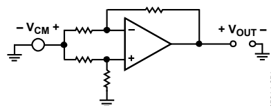
Figure 44. Common-Range Subtractor
