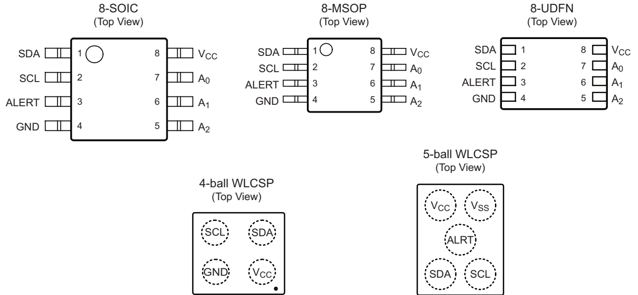
Figure 1. Pin Configurations
