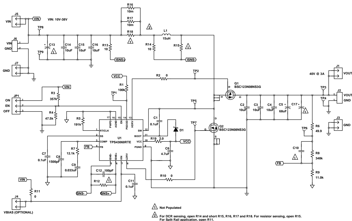
Figure 1. TPS43060EVM-199 Schematic
