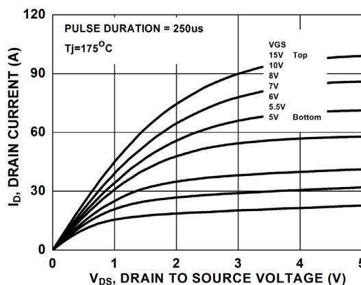
Figure 10. Saturation Characteristics
