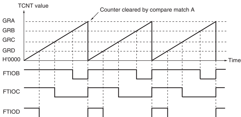
Figure 11.9 PWM Mode Example (1)
