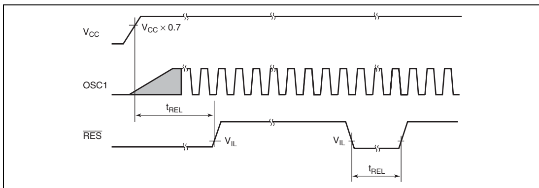
Figure 17.2 \overline{RES} Low Width Timing
