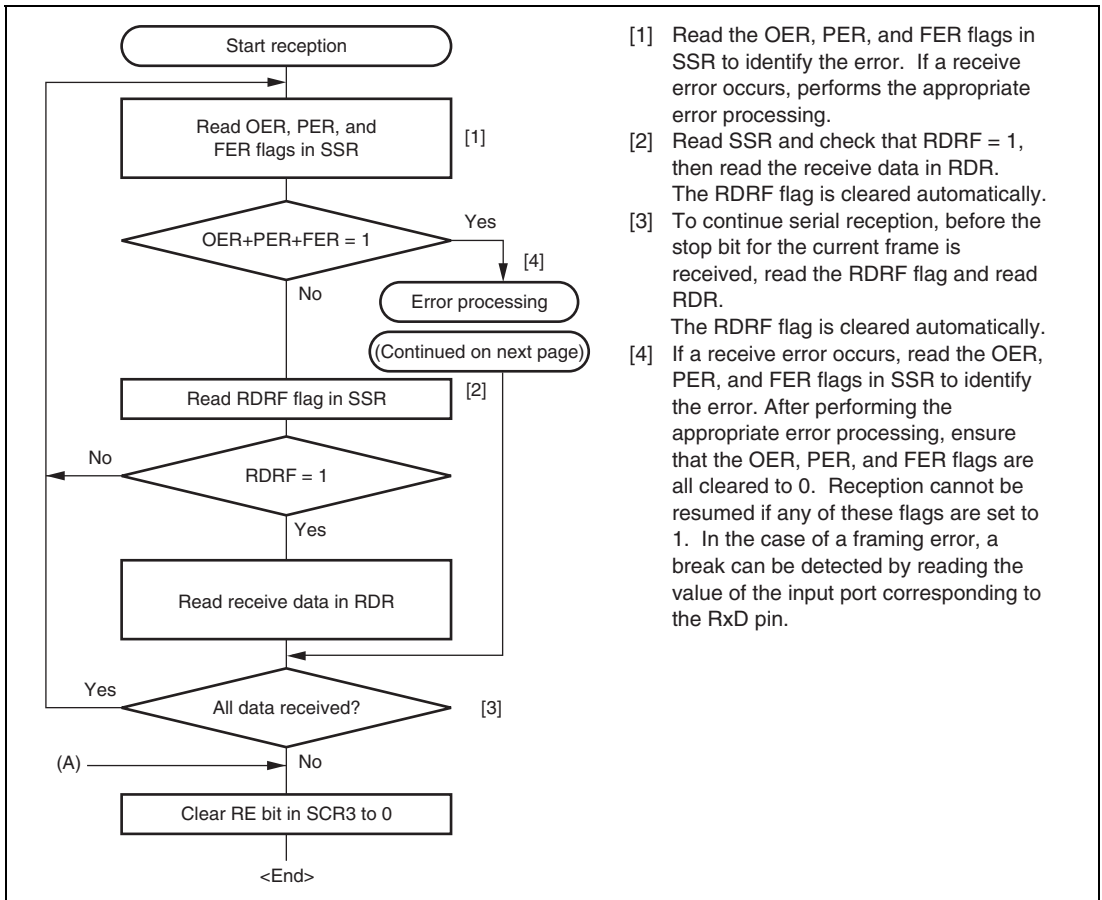
Figure 13.8 Sample Serial Data Reception Flowchart (Asynchronous mode) (1)
