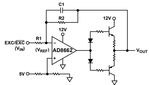
Figure 27. Buffer Circuit
