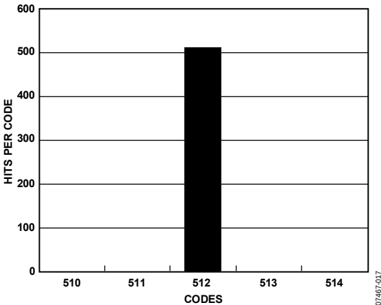
Figure 7. Typical 12-Bit Angular Accuracy Histogram of Codes, 512 Samples, Hysteresis Enabled
