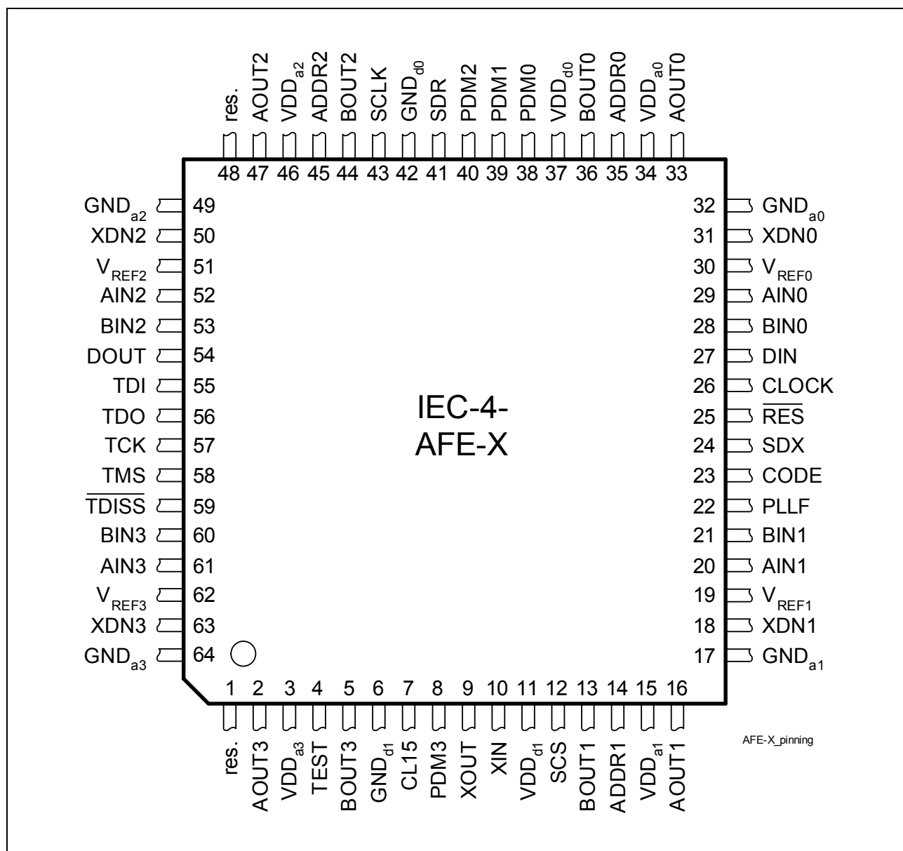
Figure 3 Pin Diagram IEC-4-AFE-X Version 3.2
