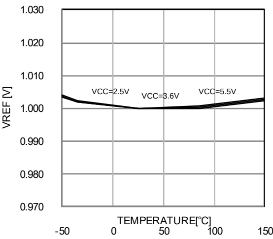
Fig.4 VREF vs temp
