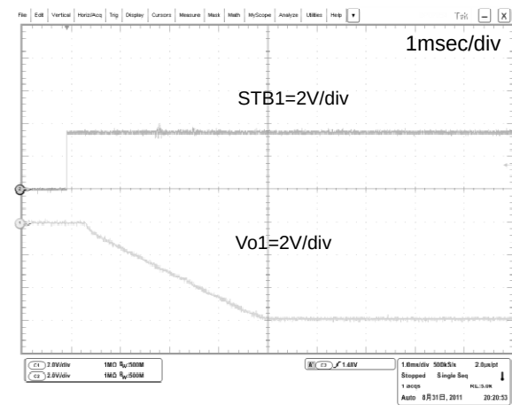
Fig.29 CH1 Soft start waveform
