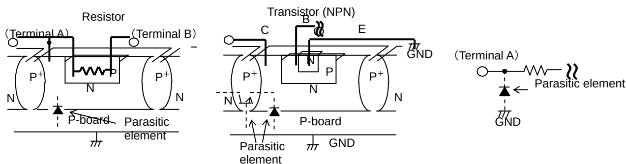
Fig.36 Simplified structure of a Bipolar IC
