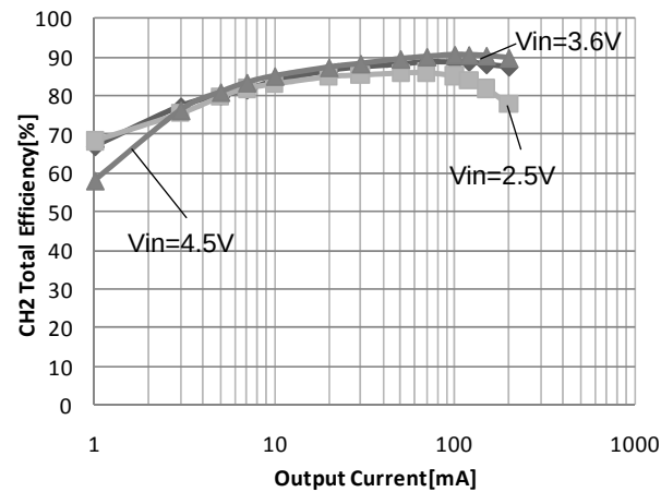
Fig.22 CH2 Power conversion efficiency vs output current
