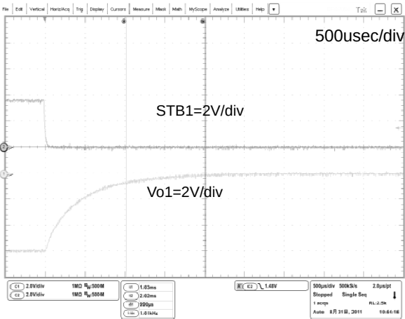
Fig.31 CH1 Discharge waveform [500usec/div] (STB1:High → Low)
