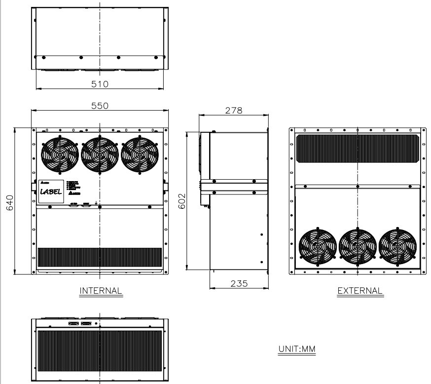
Dimension drawing
