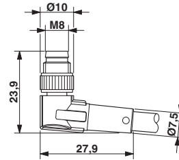
Dimensioned drawing
