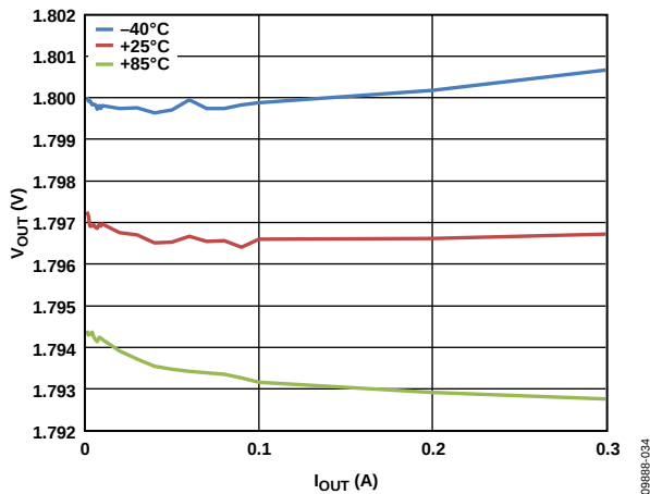
Figure 34. LDO Load Regulation Across Temperature, V_{IN3} = 3.6\text{ V} , V_{OUT3} = 1.8\text{ V}
