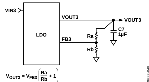
Figure 48. LDO External Output Voltage Setting
