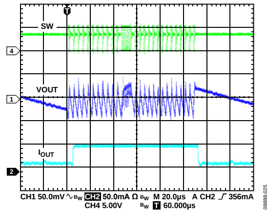
Figure 25. BUCK1 Response to Load Transient, I_{OUT1} from 1 mA to 50 mA, V_{OUT1} = 3.3\text{ V} , Automatic Mode
