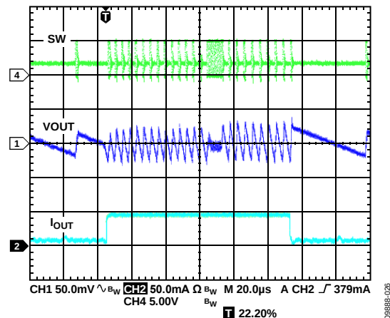
Figure 26. BUCK2 Response to Load Transient, I_{OUT2} from 1 mA to 50 mA, V_{OUT2} = 1.8\text{ V} , Automatic Mode
