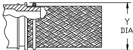
TINEL-LOCK TERMINATION
