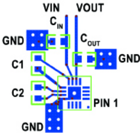
Figure 22. PCB Layout
