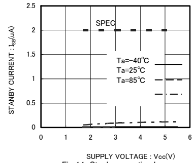
Fig.14 Standby operation I_{SB} (f scl =400kHz BR24T01/02/04/08/16/32/64/128/256-W)
