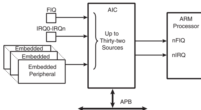
Figure 27-1. Block Diagram
