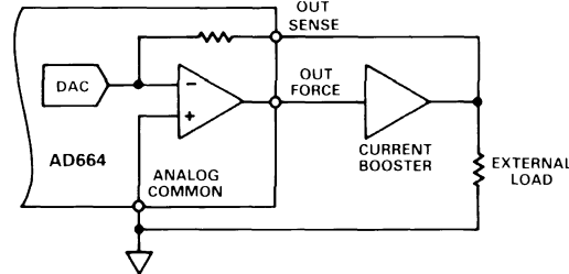
Figure 3. Current-Boosting Scheme
