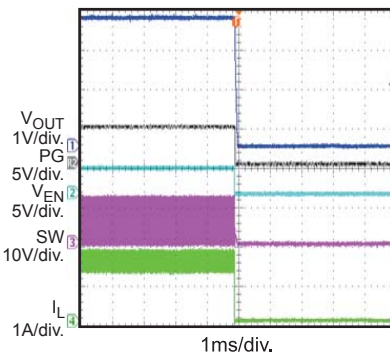
Shutdown through EN/SYNC I_{OUT}=1.5A
