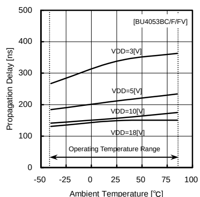
Fig.38 propagation delay time tPHZ (INH—OUT)
