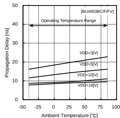
Fig.32 propagation delay time tPHL (IN—OUT)
