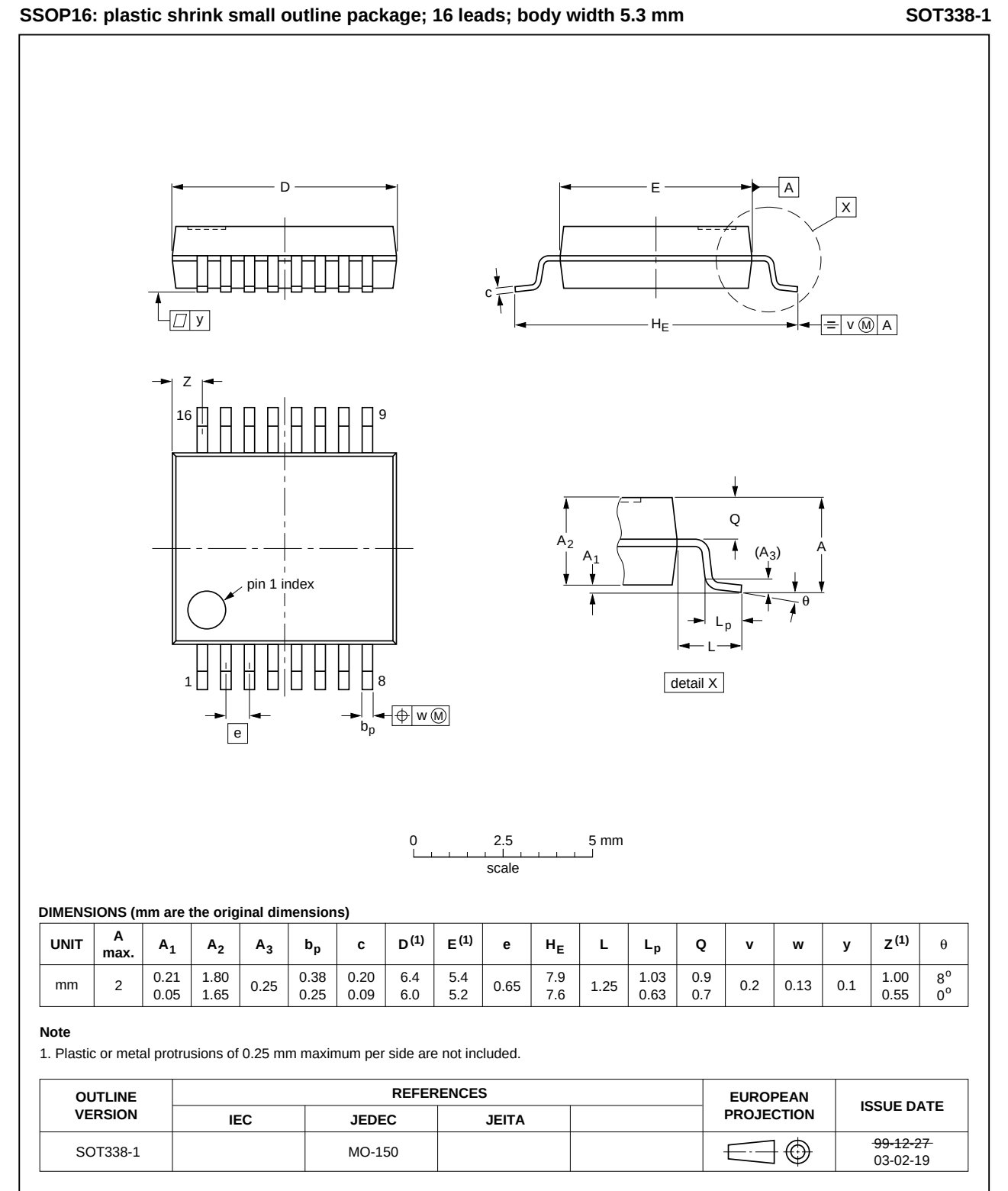
Fig 18. Package outline SOT338-1 (SSOP16)
