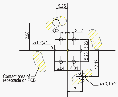
DRILLING PATTERN
