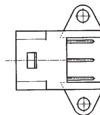
RIGHT ANGLE BOARDMOUNT FEMALE SMS--GE5 MACHINED CONTACT SMS--SE5 STAMPED CONTACT MALE SMS--GE6 MACHINED CONTACT SMS--SE6 STAMPED CONTACT
