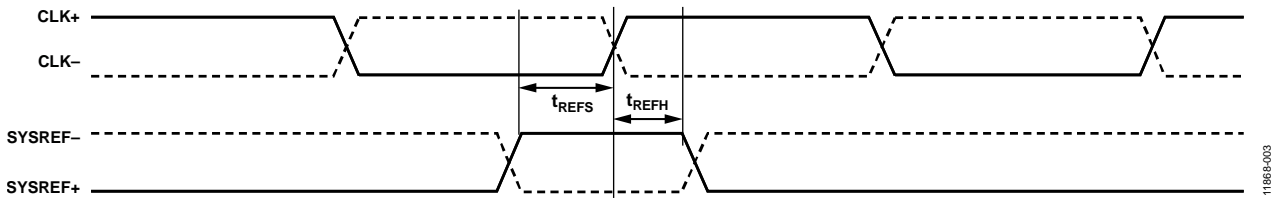
Figure 3. SYSREF_{\pm} Setup and Hold Timing (Clock Divider = 1)
