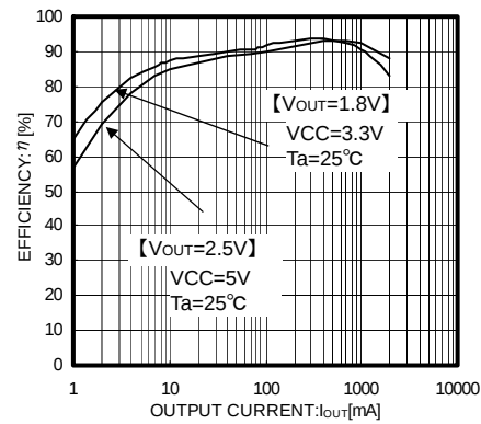
Fig.7 Efficiency
