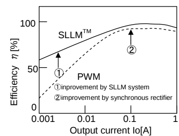
Fig.19 Efficiency
