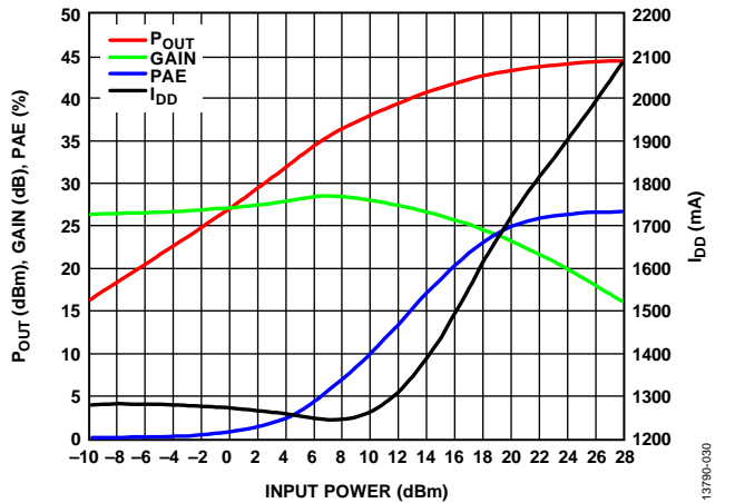
Figure 44. P_{OUT} , Gain, PAE, and Total Supply Current with RF Power Applied ( I_{DD} ) vs. Input Power, Frequency = 6 GHz
