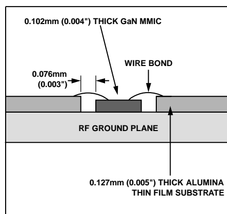
Figure 55. Die Without the Moly Tab
