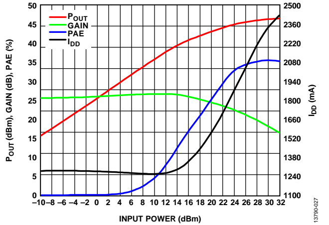
Figure 43. P_{OUT} , Gain, PAE, and Total Supply Current with RF Power Applied ( I_{DD} ) vs. Input Power, Frequency = 3 GHz
