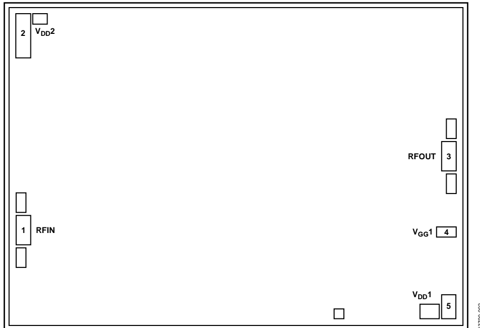
Figure 2. Pad Configuration
