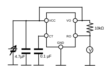
Measurement Circuit for Figure.16, 17
