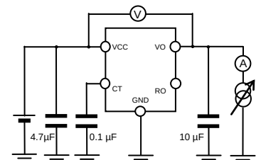
Measurement Circuit for Figure.13
