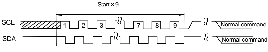
Figure 34.-(c) STARTx9 + command input
