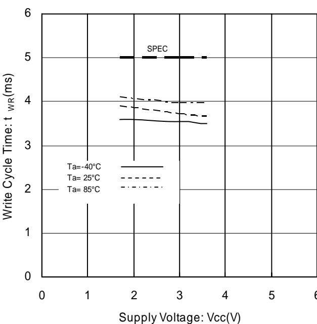
Figure 23. Write Cycle Time vs Supply Voltage
