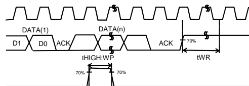
Figure 1.-(e). WP Timing at Write Cancel
