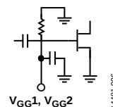
Figure 6. V GG1 , V GG2 Interface Schematic
