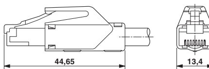
Dimensioned drawing
