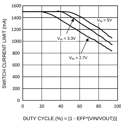
Figure 29. Switch Current Limit vs Duty Cycle - “Y”
