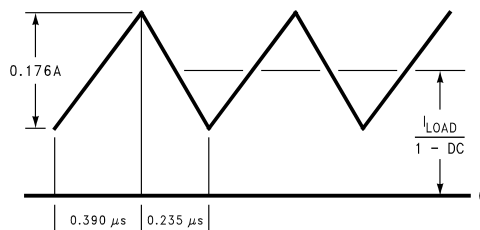
Figure 27. 10 \mu H Inductor Current, 5V–12V Boost (LM2733X)
