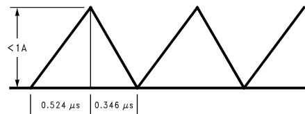
Figure 32. Discontinuous Design, 5V-12V Boost (LM2733X)
