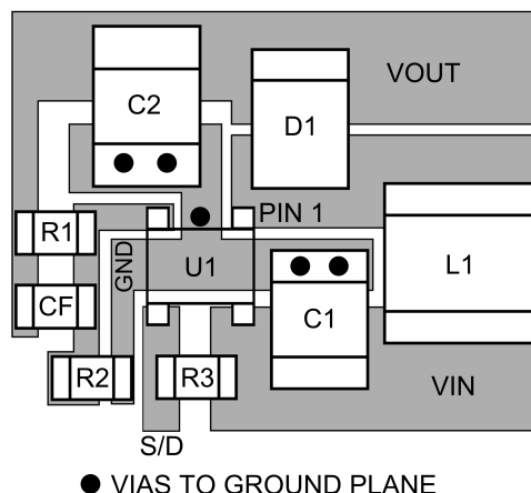
Figure 25. Recommended PCB Component Layout
