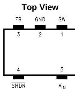
Figure 1. 5-Lead SOT-23 Package See Package Number DBV (R-PDSO-G5)
