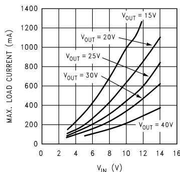
Figure 31. Max. Load Current vs V IN - "Y"
