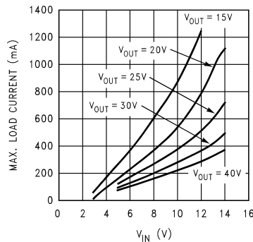
Figure 30. Max. Load Current vs V IN - "X"
