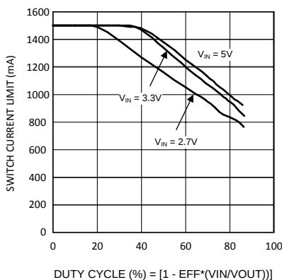
Figure 28. Switch Current Limit vs Duty Cycle - “X”
