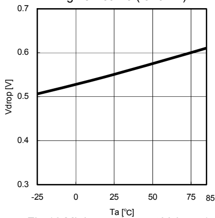
Fig.16 Minimum dropout Voltage 1 ( V_{cc}=5\text{V} , I_o=-1.5\text{A} )
