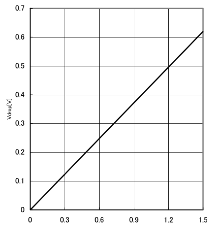
Fig.20 Minimum dropout Voltage 2 ( V_{cc}=4.5\text{V} , T_a=25^\circ\text{C} )
