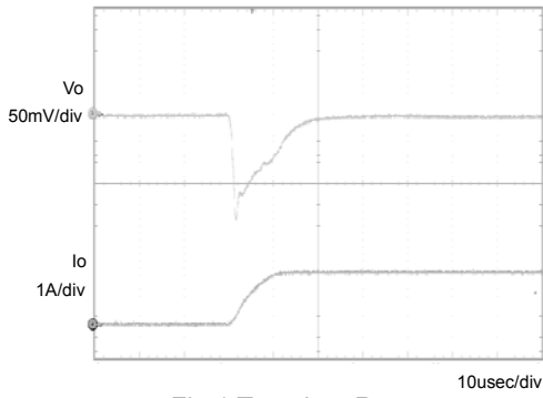
Fig.1 Transient Response (0→1.5A) C_o=1\mu\text{F}
