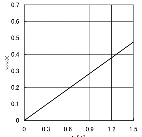
Fig.21 Minimum dropout Voltage 3 ( V_{cc}=6V , T_a=25^\circ C )
