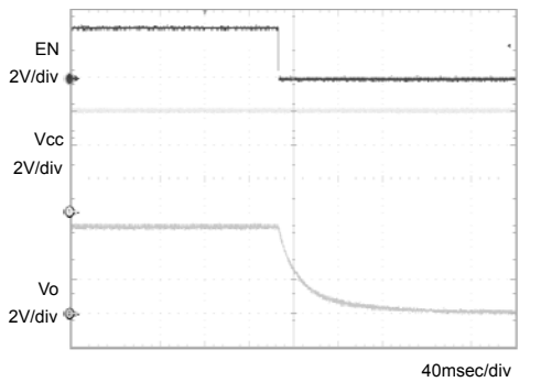
Fig.6 OFF sequence 2 C_o=1\mu\text{F}
