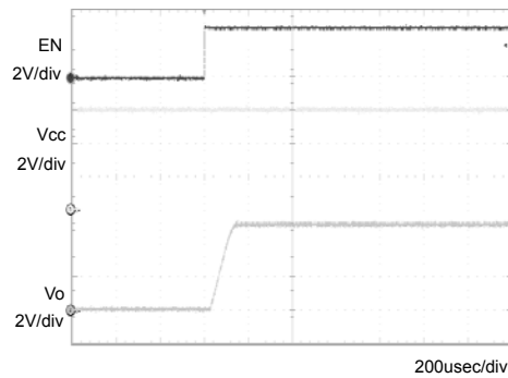
Fig.5 Input sequence 2 C_o=1\mu\text{F}
