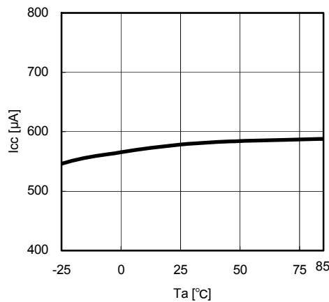
Fig.8 T_a - I_{CC}
