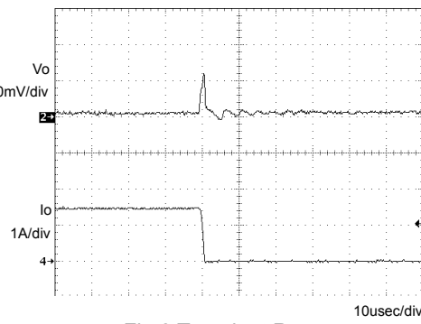
Fig.2 Transient Response (1.5→0A) C_o=1\mu\text{F}
