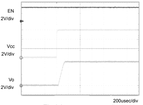
Fig.3 Input sequence 1 C_o=1\mu\text{F}
