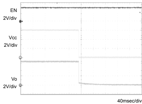
Fig.4 OFF sequence 1 C_o=1\mu\text{F}
