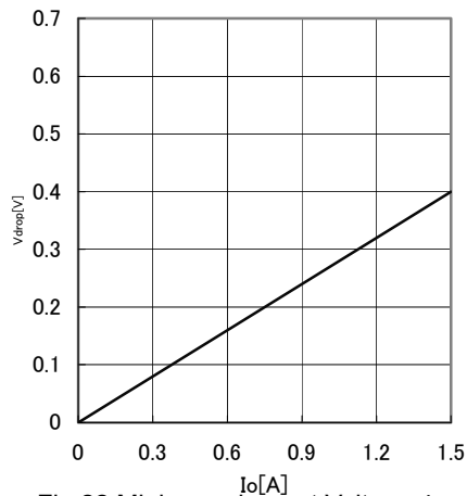
Fig.22 Minimum dropout Voltage 4 ( V_{cc}=8V , T_a=25^\circ C )
