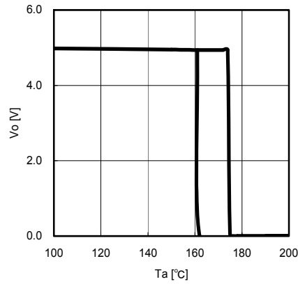
Fig.14 TSD ( I_o=0mA )
