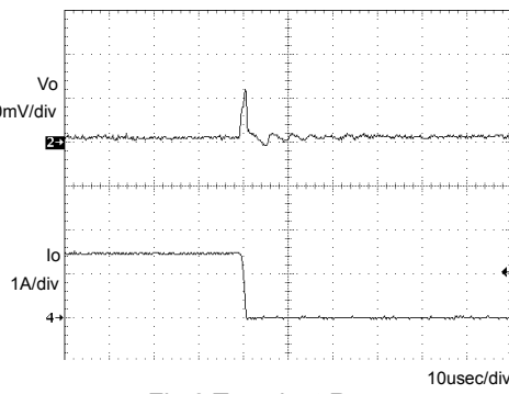
Fig.2 Transient Response (1.5→0A) C_o=1\mu\text{F}
