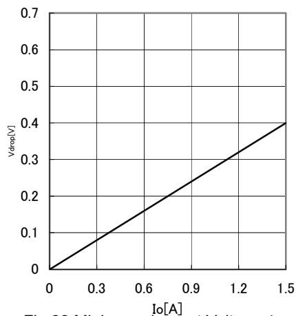
Fig.22 Minimum dropout Voltage 4 ( V_{cc}=8V , T_a=25°C )
