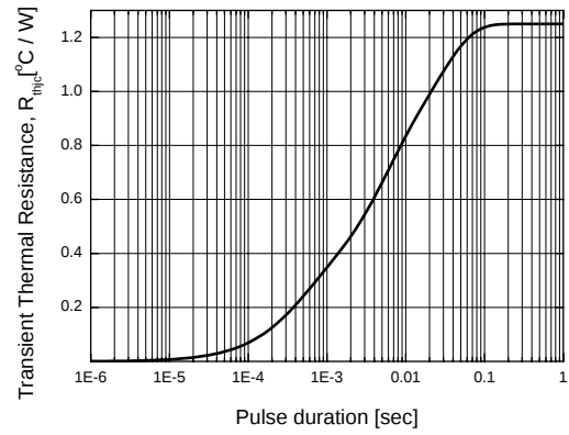
Figure 8. Thermal Resistance
