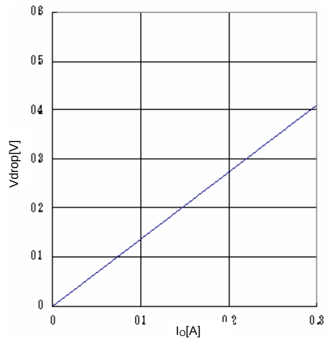
Fig.22 Minimum dropout Voltage 2 ( V_{CC}=4.5 V, T_a=25^{\circ} C)
