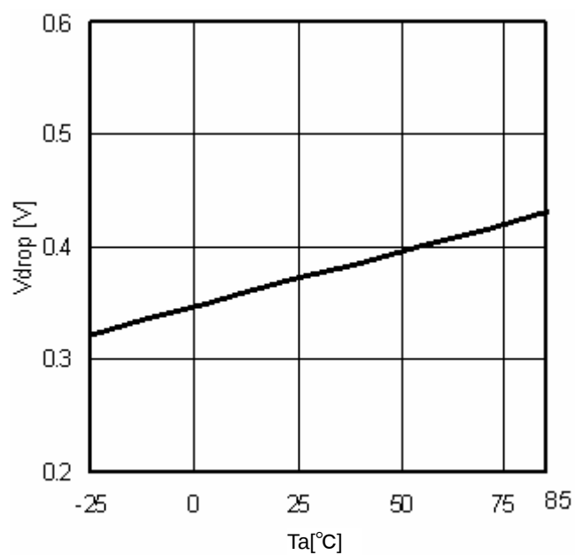
Fig.18 Minimum dropout Voltage ( V_{CC}=5\text{V} , I_O=-0.3\text{A} )
