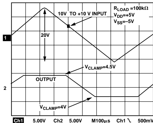
Figure 6. Overvoltage Ramp
