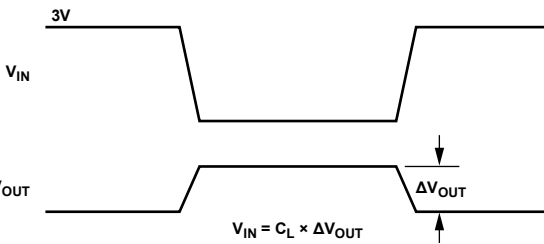
Figure 21. Charge Injection
