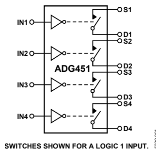
Figure 1. ADG451
