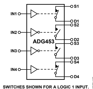
Figure 3. ADG453
