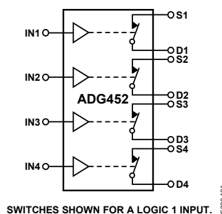
Figure 2. ADG452
